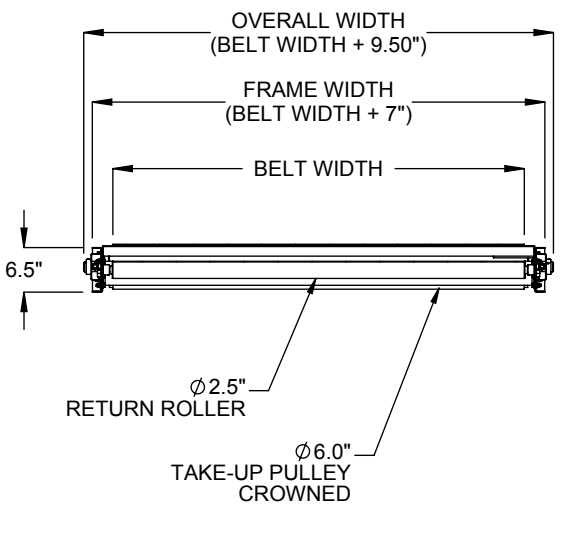
SECTION A-A TAKE-UP END TYP ALL DRIVES
