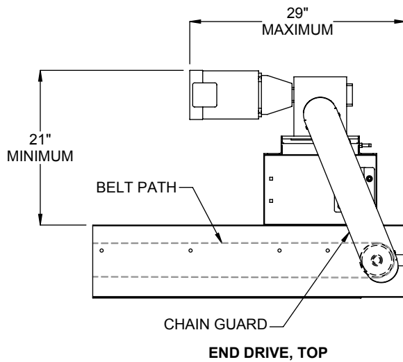
END DRIVE, TOP
