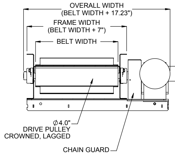
SECTION B-B DRIVE END
