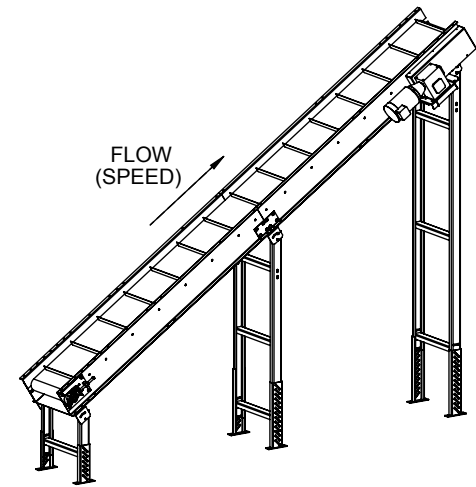
END DRIVE, SIDE, RIGHT HAND (SHOWN) END DRIVE, SIDE, LEFT HAND (OPPOSITE)
