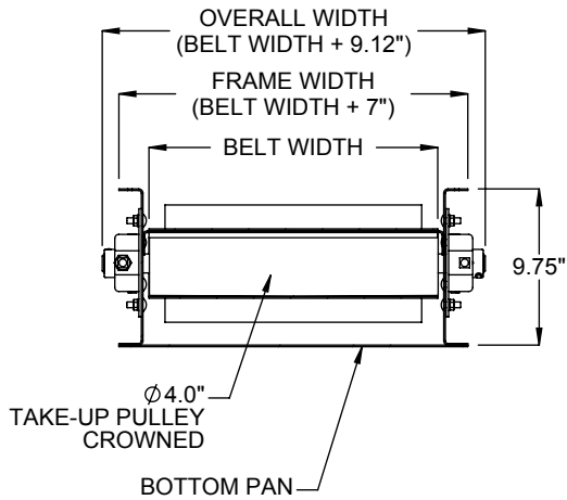
SECTION A-A TAKE-UP END TYPICAL ALL DRIVES
